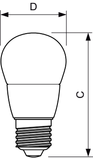
Candle 230V 8-60W 806lm 2700K E27 ND FR
